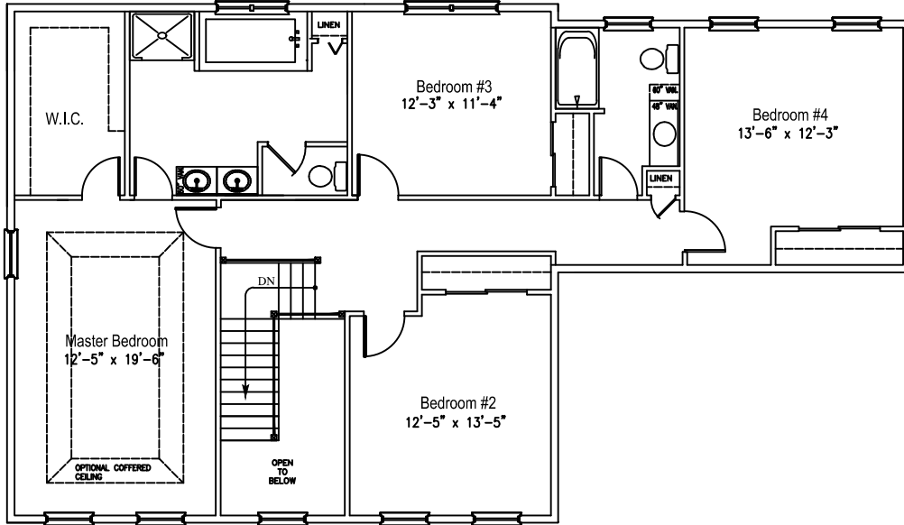
EMERSON 1 SECOND FLOOR
