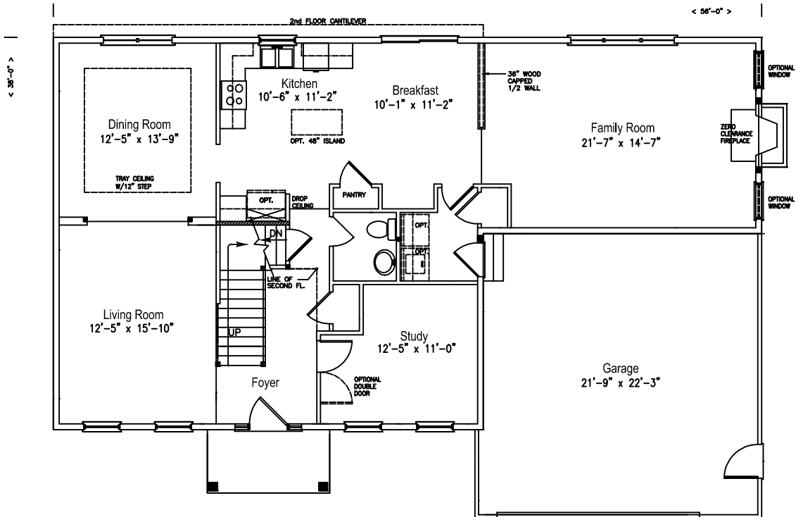
EMERSON 1 FIRST FLOOR
