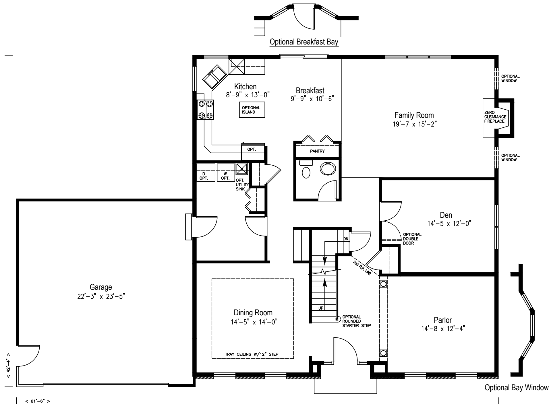
HAWTHORNE 1 FIRST FLOOR
