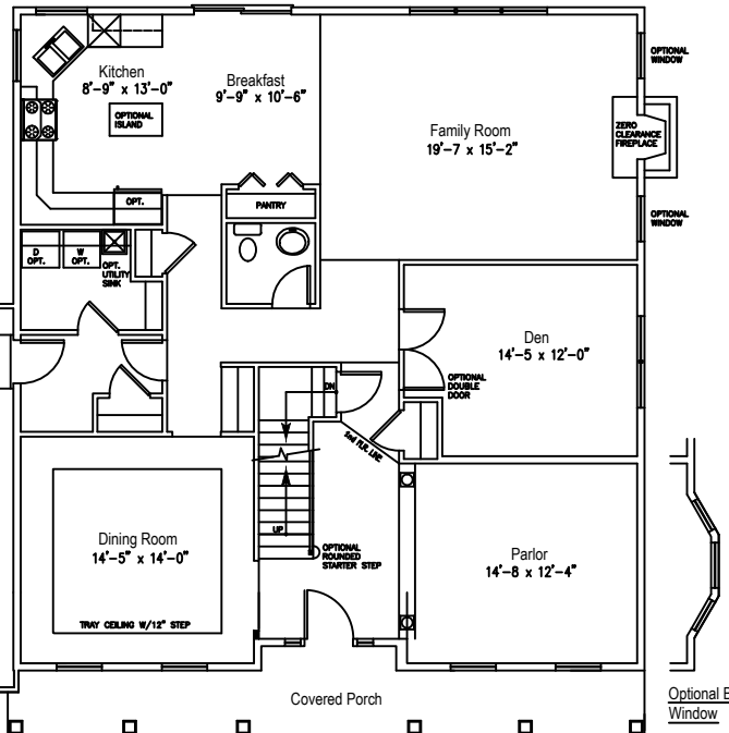
HAWTHORNE 2 FIRST FLOOR
