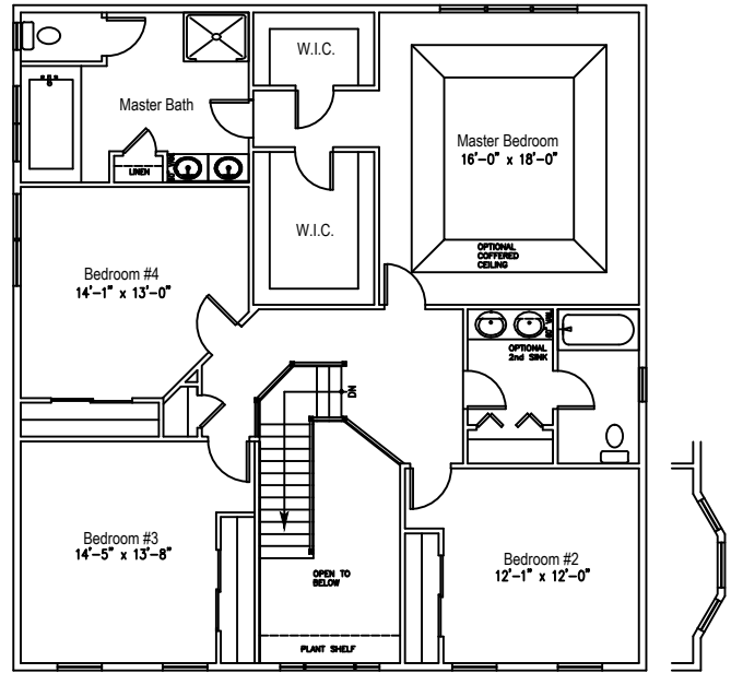
HAWTHORNE 2 SECOND FLOOR
