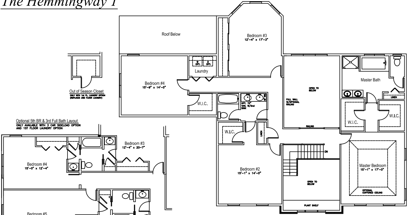
HEMMINGWAY 1 SECOND FLOOR
