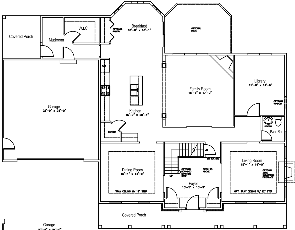
HEMMINGWAY 1 FIRST FLOOR
