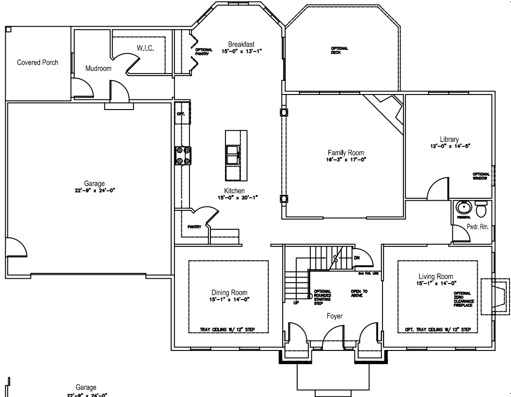
HEMMINGWAY 3 FIRST FLOOR
