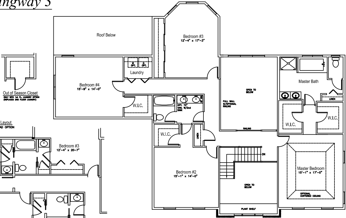
HEMMINGWAY 3 SECOND FLOOR
