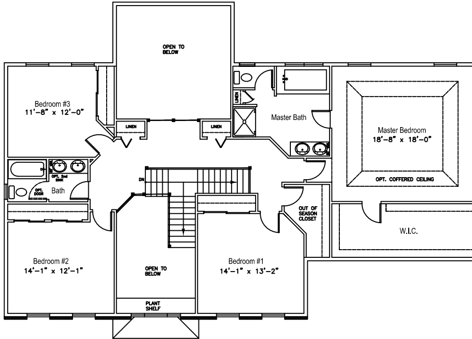
STEINBECK 1 SECOND FLOOR
