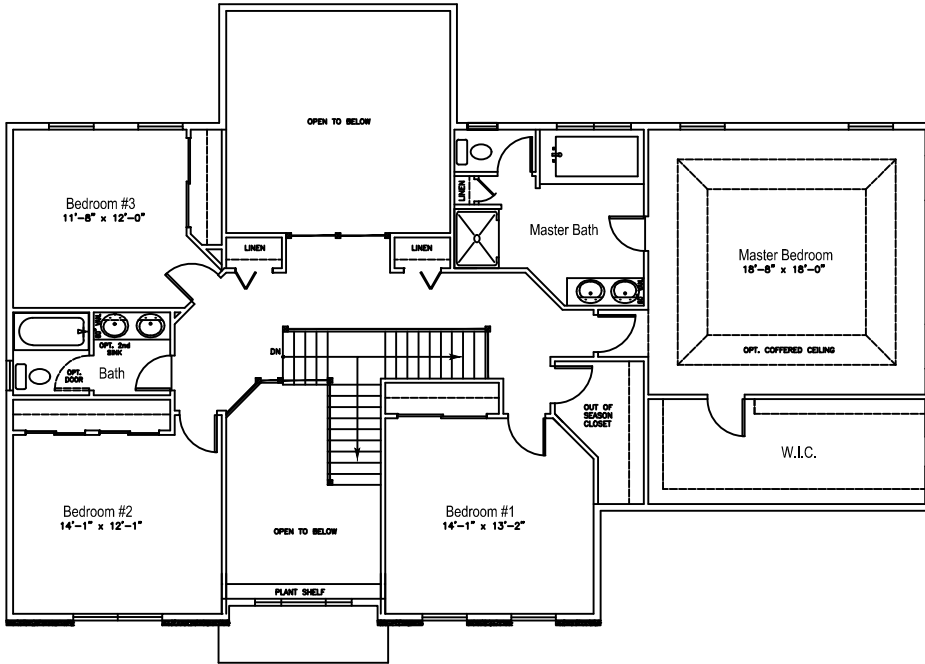
STEINBECK 3 SECOND FLOOR
