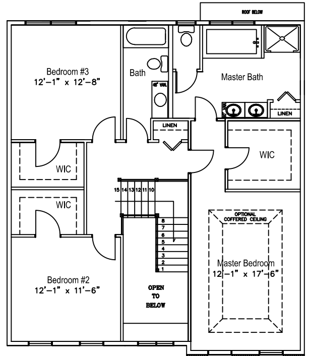
Windsor 1 Second Floor Plan
