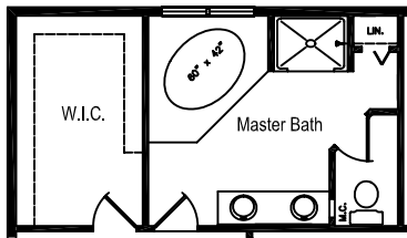
Master Bath 4'-0" Shower Option AVAILABLE W/OPEN FOYER OPTION ONLY
