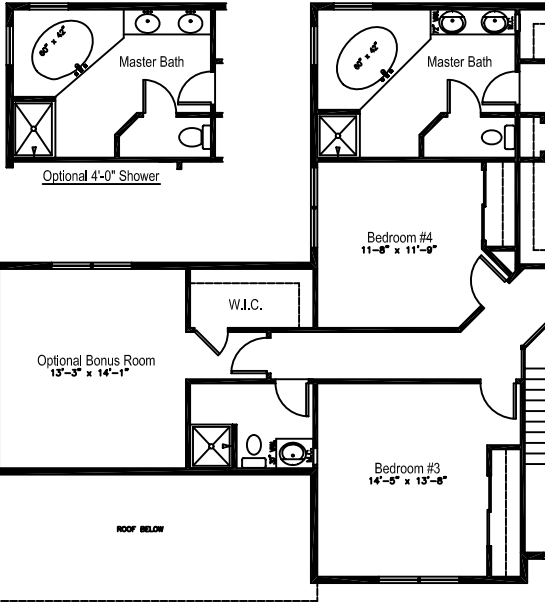
Optional Bonus Room with Third Bath ADDITIONAL 344 sq. ft.
