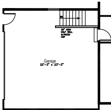
Side Load Garage Option SHOWN WITH OPTIONAL REAR WINDOW AND BASEMENT STAIRS
