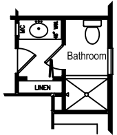
Optional Main Bath Layout w/4'-0" Shower
