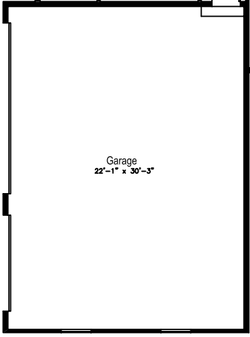
Three Car Side Load Garage Option ELIMINATES SERVICE DOOR
