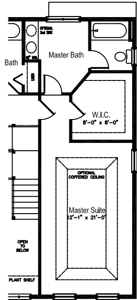
Master Bath Option
