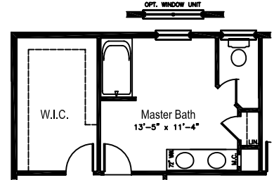
Master Bath Option for Optional Open Foyer
