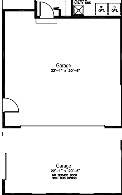
Side Load Garage Option
